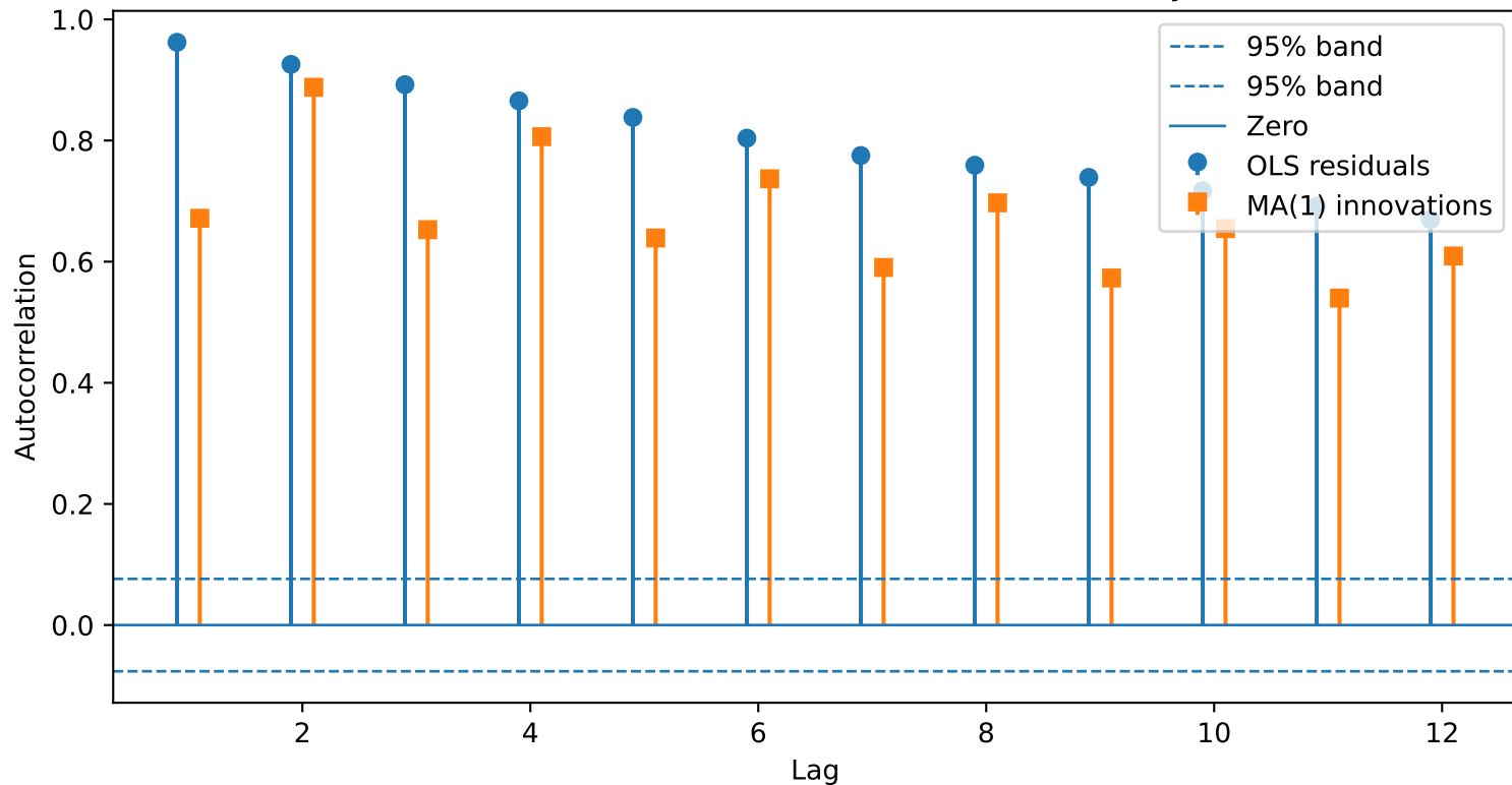
Dataset 1 - Residual ACF: OLS vs recursive MA(1) Taylor rule
